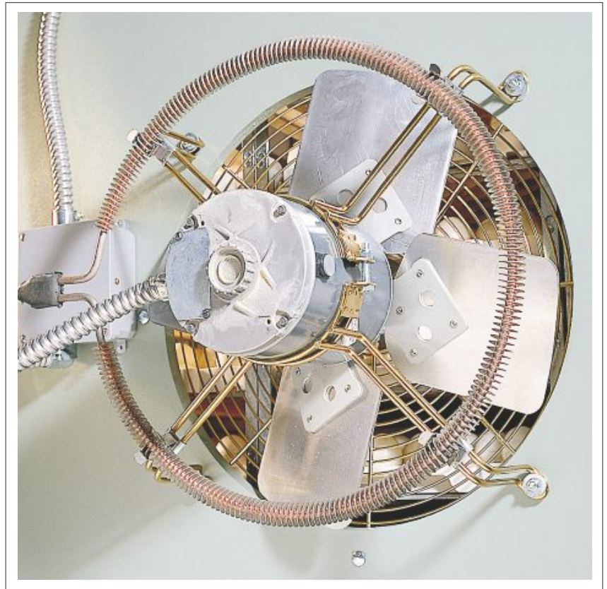
New ring heating element mounted on the fan
