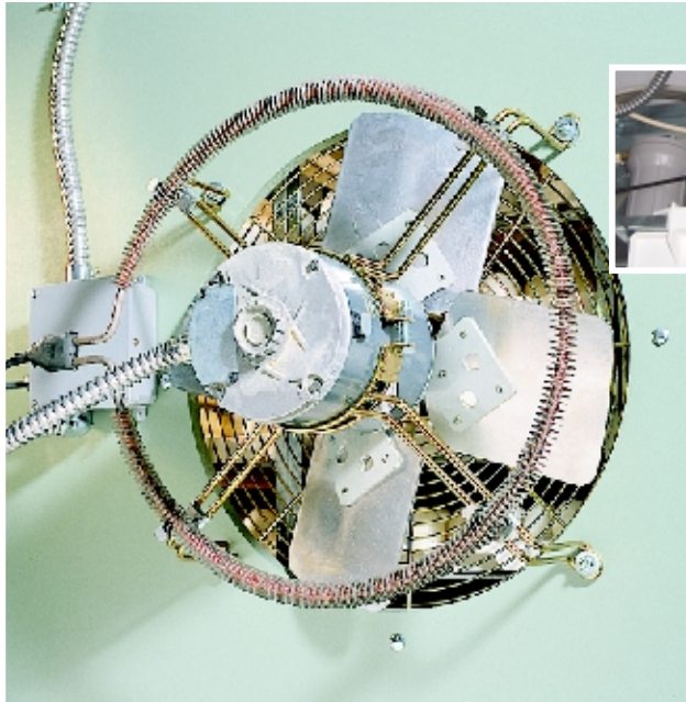
NEW RING HEATING ELEMENT MOUNTED ON THE FAN
