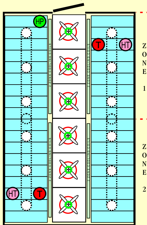
C576-165 Classic Setter Internal Layout
