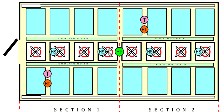
B16D-120 Multi-Stage Roll-In Duck Setter Internal Layout
