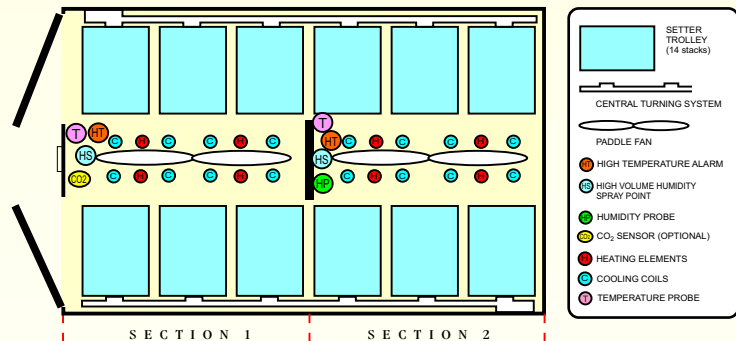
A12D-120 Single-Stage Duck Setter Internal Layout
